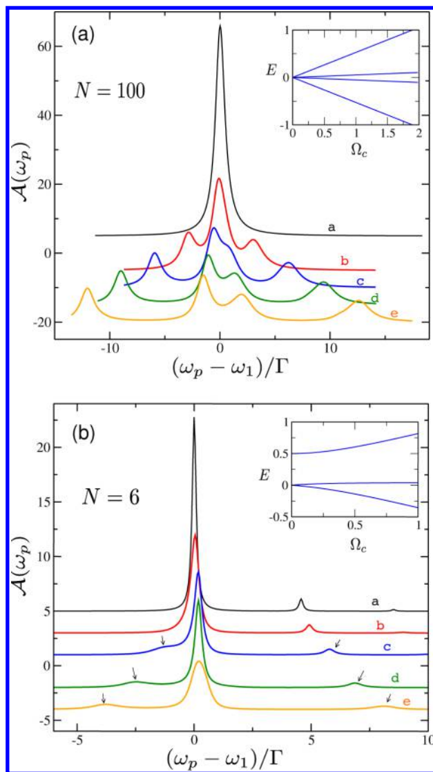
Figure 2. Probe absorption spectrum \mathcal{A}(\omega_p) = -\text{Im}[\chi] (in units of \epsilon_0/\hbar ) as a function of the detuning from the lowest exciton resonance \Delta_1 = \omega_p - \omega_1 (in units of the decay rate \Gamma = 26 meV) for an ideal open linear polar J-aggregate of size N in a microcavity (no energetic disorder). (a) N = 100 . Curves are labeled according to the mean cavity amplitude A_c \equiv |\langle a \rangle| as (a) no cavity, (b) A_c = 0.2 , (c) A_c = 0.4 , (d) A_c = 0.6 , and (e) A_c = 0.8 . The inset shows the eigenvalues of the four-level effective Hamiltonian in eq 8 with \Delta_2 = 0 = \Delta_{23} and \Omega_1 = \Omega_2/3 = 3\Omega_3 as a function of \Omega_c = \Omega_2 (in arbitrary units). (b) N = 6 . Curves are labeled by the value of A_c as (a) no cavity, (b) A_c = 0.4 , (c) A_c = 0.8 , (d) A_c = 1.2 , and (e) A_c = 1.6 . The inset shows the eigenvalues of eq 8 with \Delta_2 = 0.5 , \Omega_1 = \Omega_2/3 , and \Omega_3 = 0 as a function of \Omega_c = \Omega_2 . In both panels, the cavity frequency is resonant with the transition |k_1\rangle \rightarrow |k_1 k_2\rangle .
